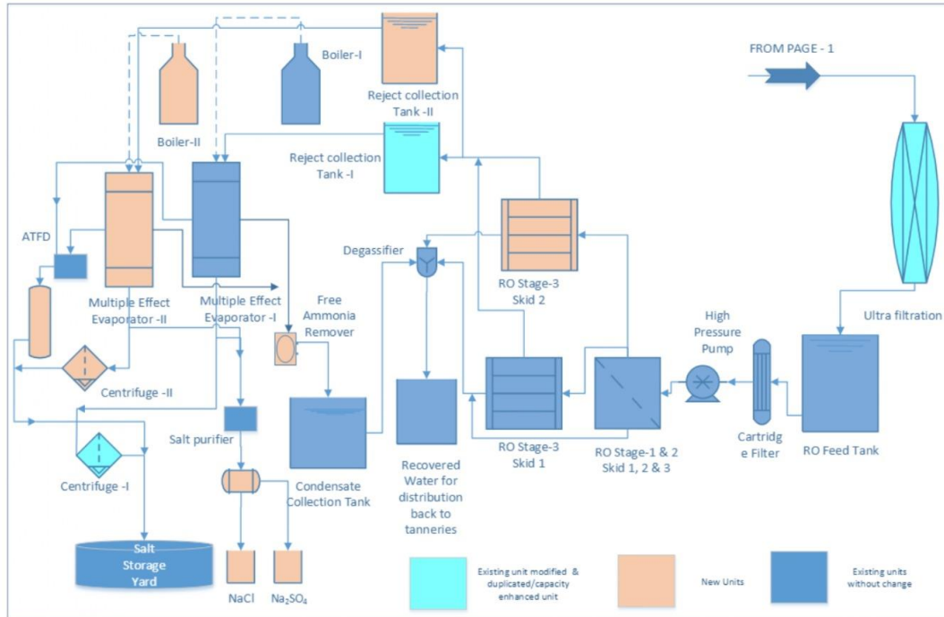
RANITEC CETP schematic Process Flow Diagram showing existing and upgraded units
