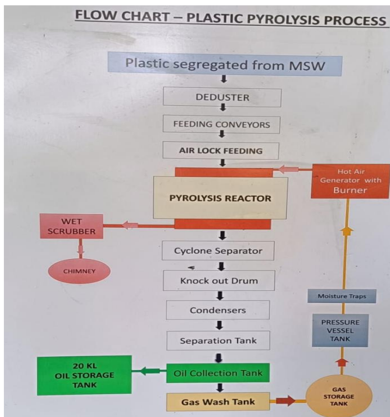
Figure 54: Nashik Plastic to Fuel
