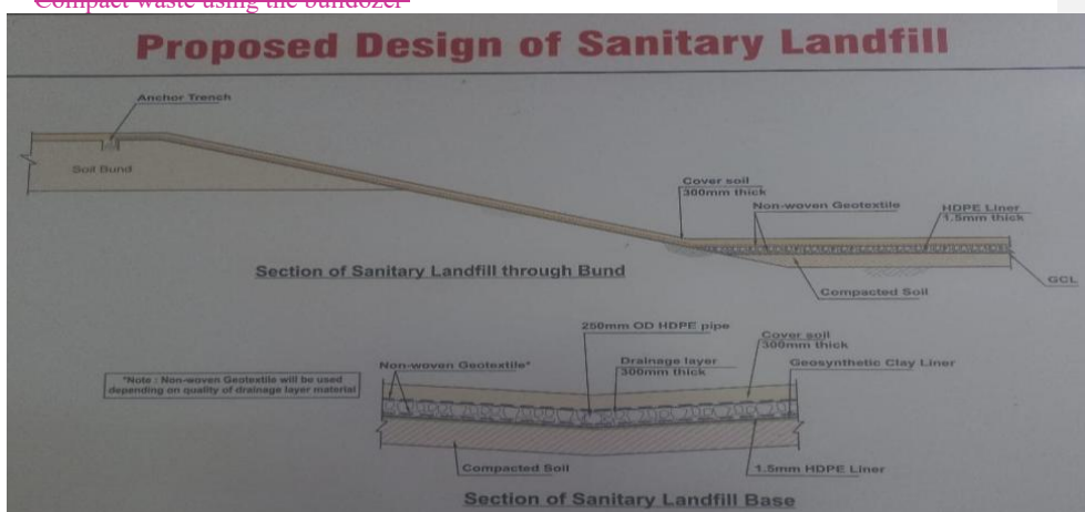
Figure 6-7: Reject to Landfill (SLF)
