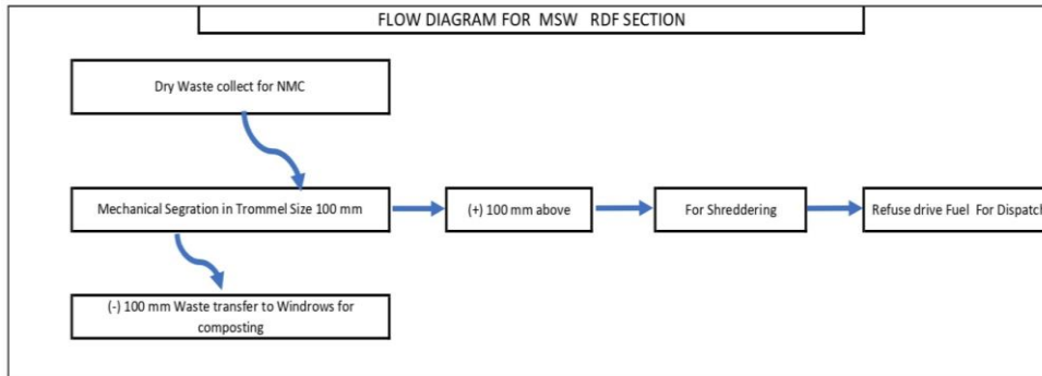
Figure 2 : RDF Production
