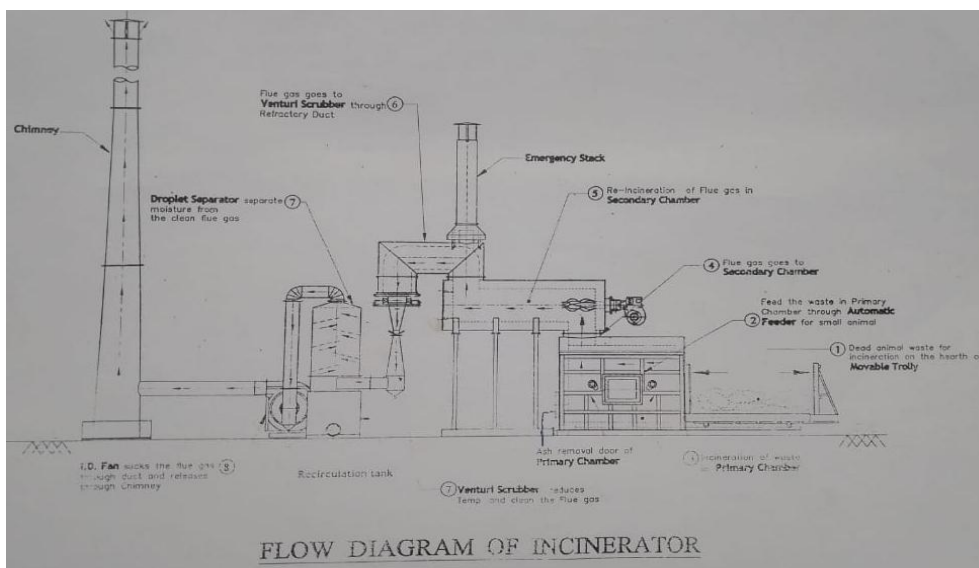
Figure 56: Dead Animal Incineration
