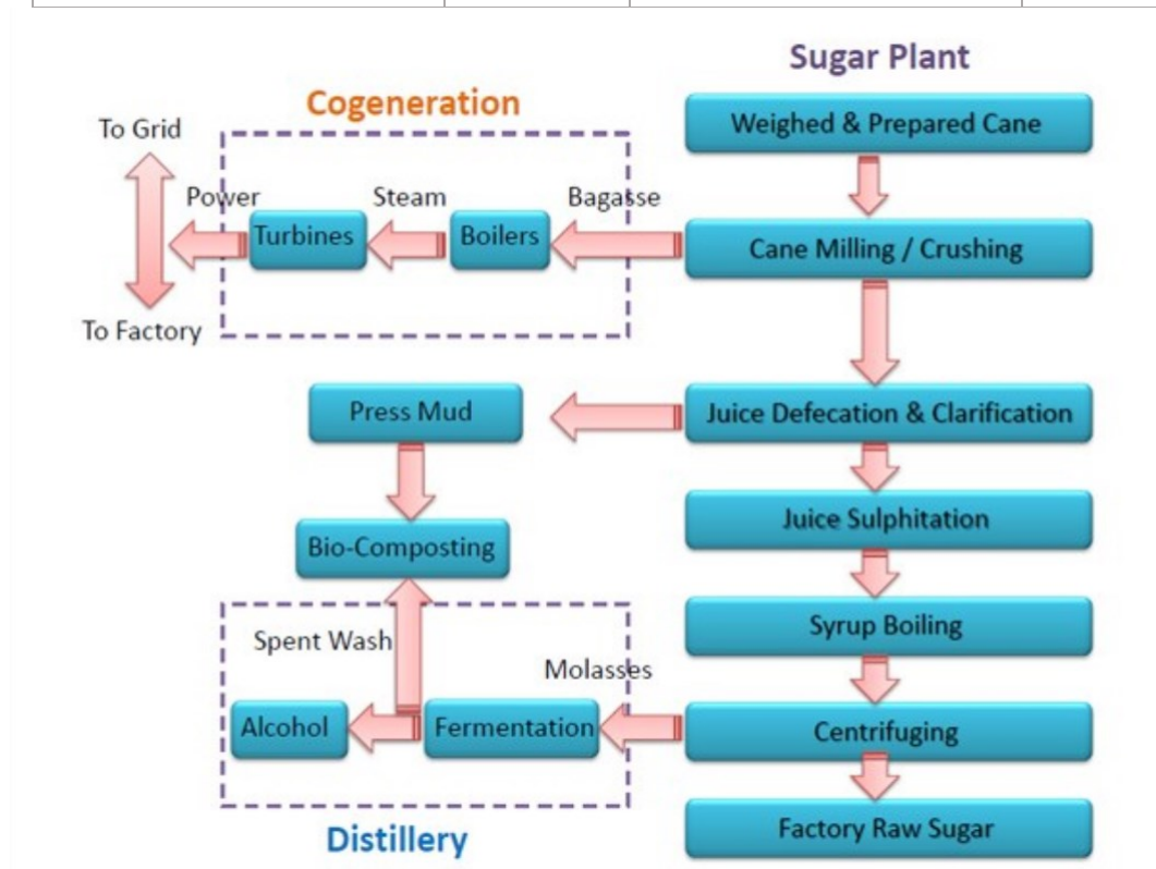
Figure 4-Sugar & Co-gen power plant process flow chart
